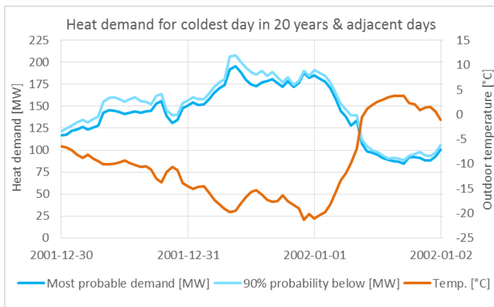
Figure 21. Heat demand profile for coldest day in 20 years and adjacent days. The design heat demand for the upper confidence interval and hence the required capacity is 208 MW
