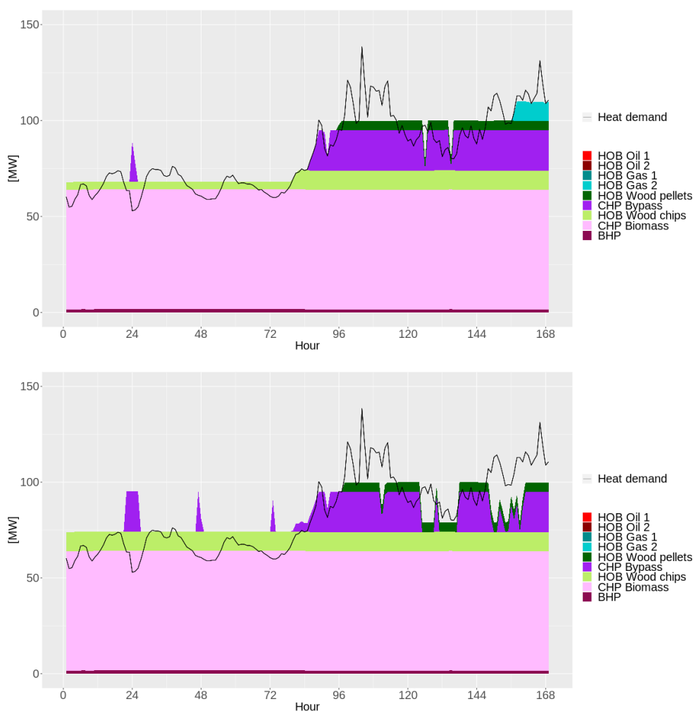
Figure 9. Heat generation during a November week in 2016 for archetype heat grid: CHP S
