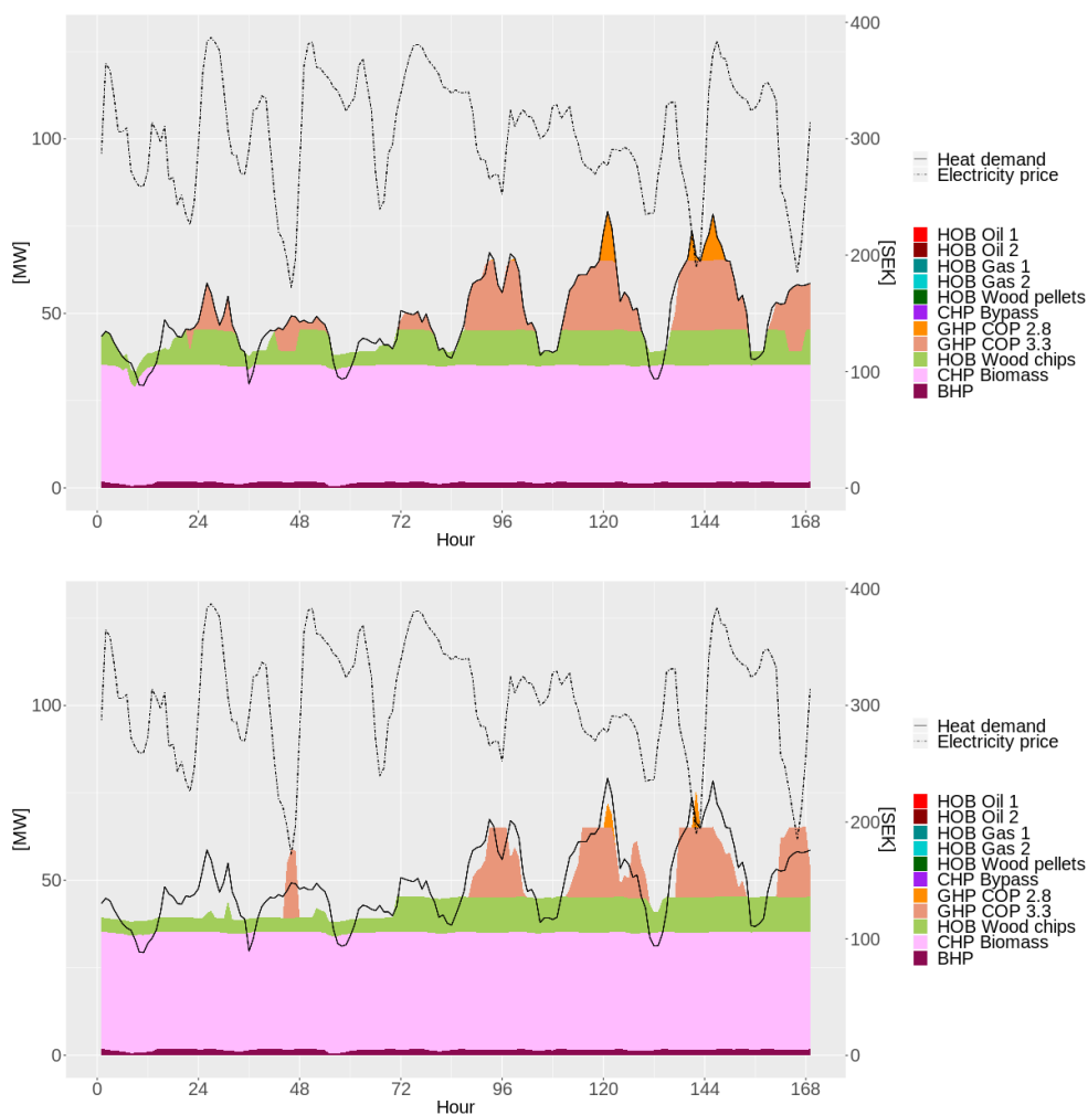
Figure 10. Heat generation during an April week in 2015 for archetype heat grid: GHP
