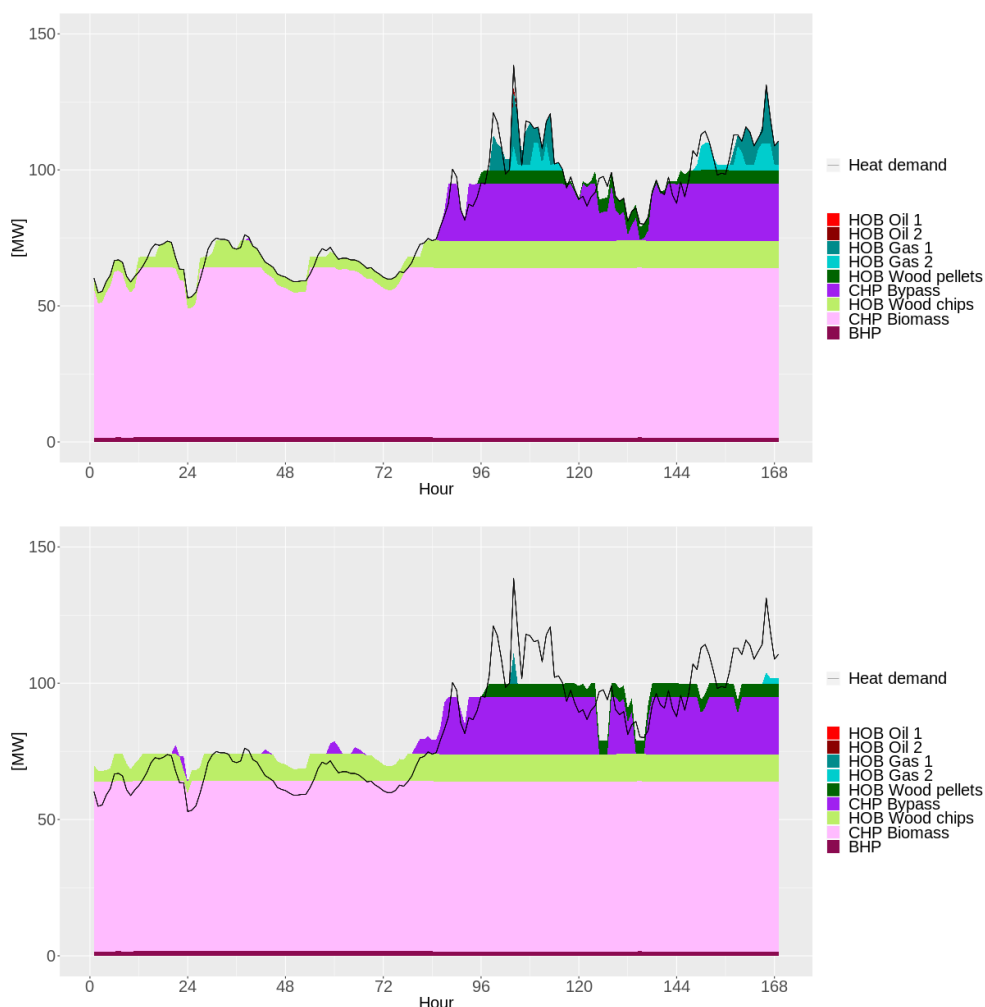
Figure 8. Heat generation during a November week in 2016 for archetype heat grid CHP
