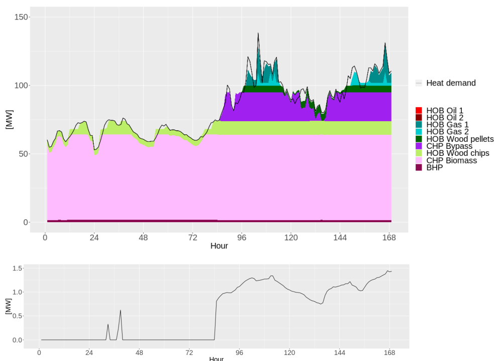
Figure 16. Upper figure: Heat generation from all heat sources during one week in November 2016 for case:
