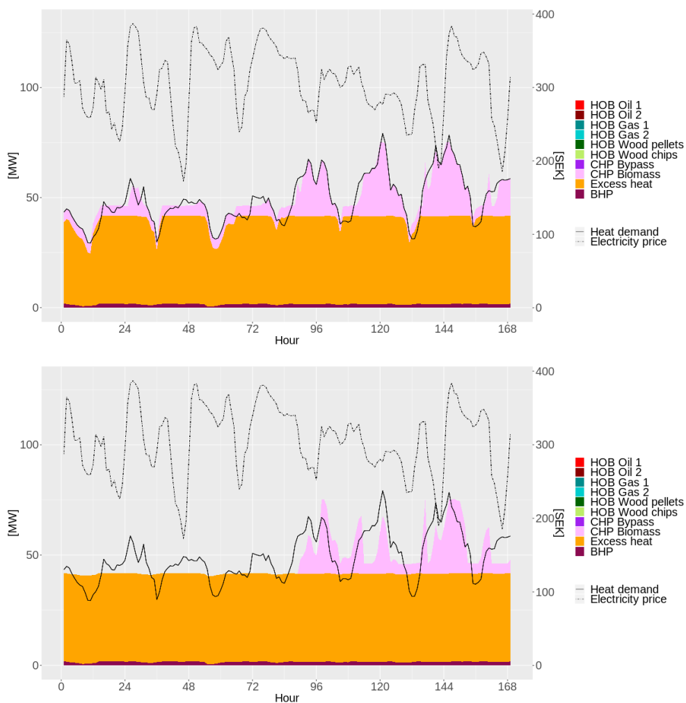
Figure 11. Heat generation during an April week in 2015 for archetype heat grid: EH
