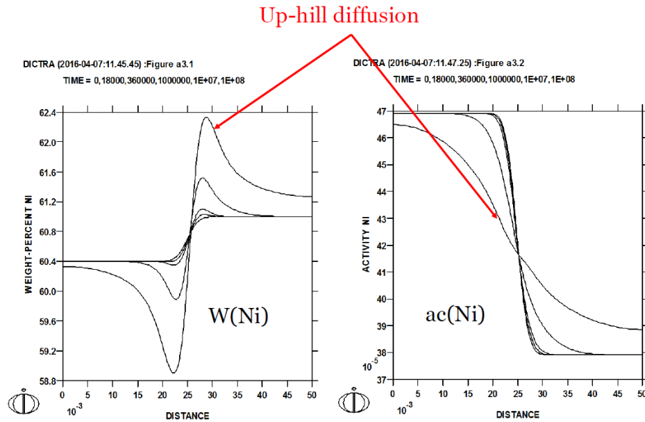
Figure 17 Simulation results of Ni-concentration profile (left) and Ni-activity (right) showing increase of Ni concentration near the coating-substrate interface with time through uphill diffusion.
