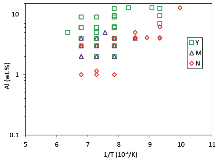
Figure 19 A summary of literature data relating showing the Al-concentration and oxidation stage. \square Y: alloys able to form a single scale of alumina, \triangle M: alloys able to form an alumina scale with other oxides outside, \diamond N: alloys unable to form a continuous alumina and severe internal oxidation occurs.
