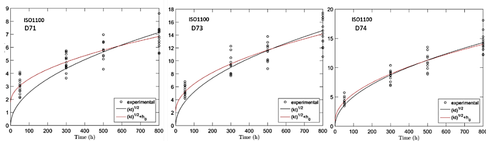
Figure 2 TGO thickness of three Fe-containing coatings during isothermal oxidation at 1100 °C.
