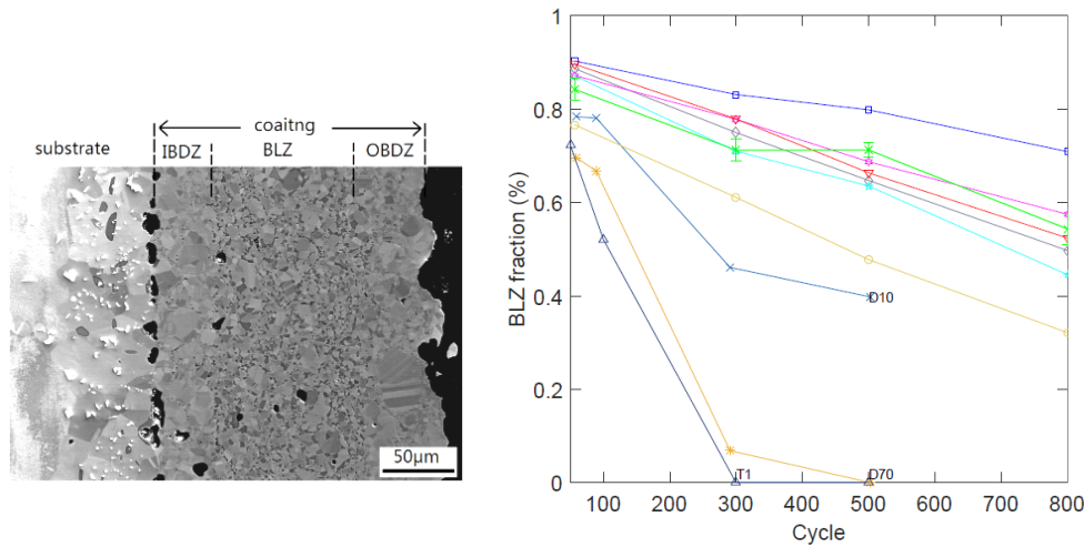
Figure 1 Definition of the different microstructural layer (left) and comparison of resistance to \beta -depletion between the Ni-base coatings under TCF (D1x and D7x).
