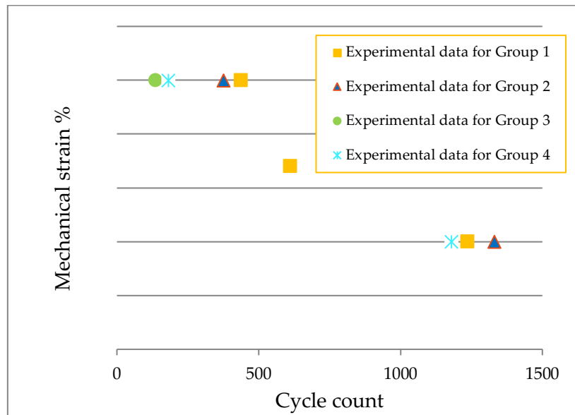
Figure 13 Comparison of TMF life between D10, D11, and D71 (Group 1, 2, and 3 respectively) coated IN792. Group 4 is the uncoated IN792.
